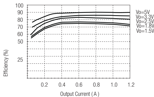
Efficiency Vs Load (Vin=Max)
